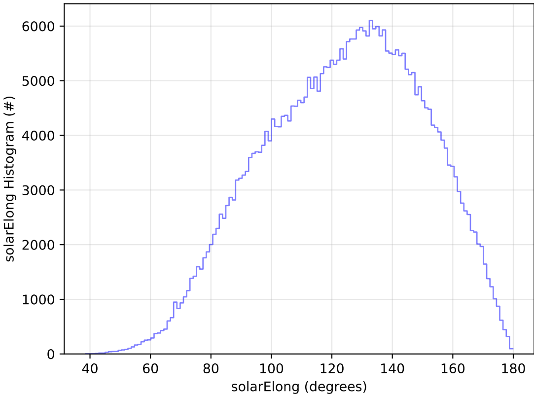
too_elab_r128_d2_gz_v3.4_10yrs All sky y band: solarElong Histogram
