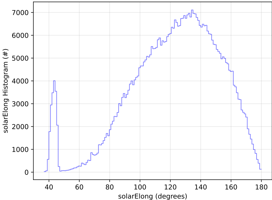
too_elab_r128_d2_gz_v3.4_10yrs All sky r band: solarElong Histogram
