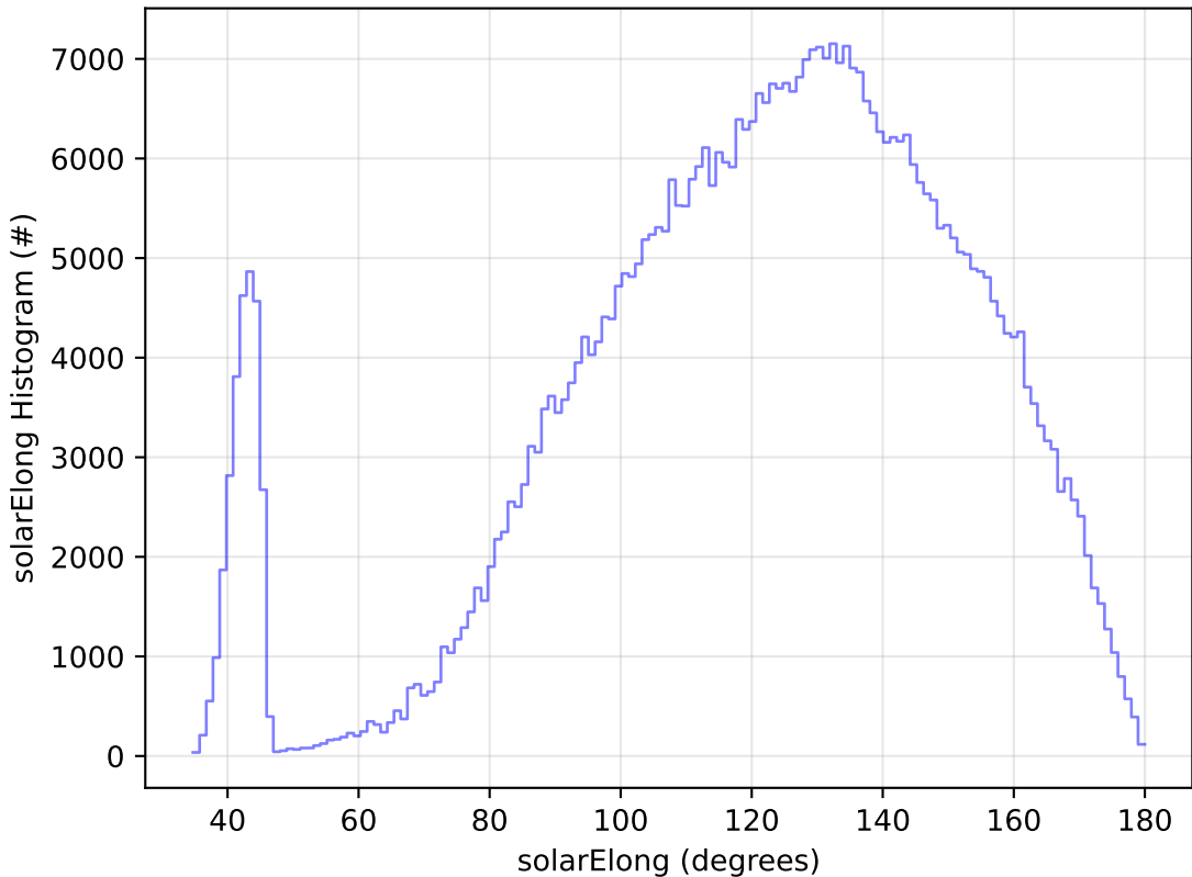
too_elab_r128_d2_gz_v3.4_10yrs All sky i band: solarElong Histogram
