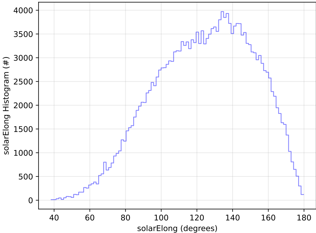
too_elab_r128_d2_gz_v3.4_10yrs All sky g band: solarElong Histogram
