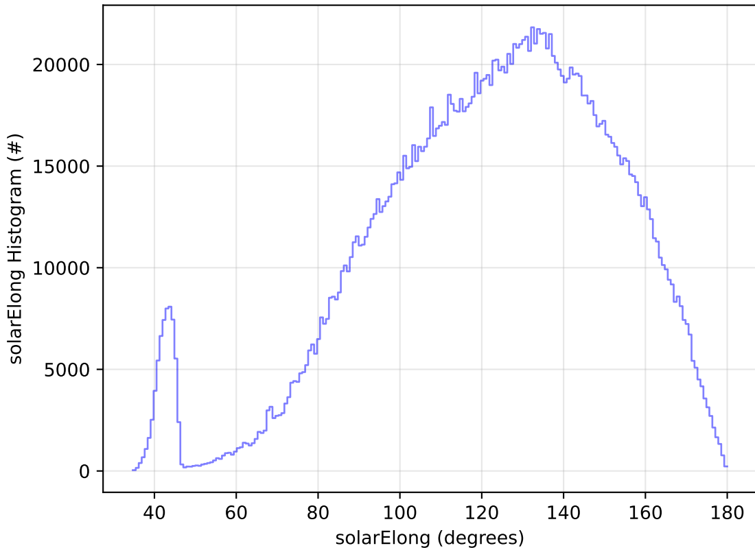
too_elab_r128_d2_gz_v3.4_10yrs All sky all bands: solarElong Histogram
