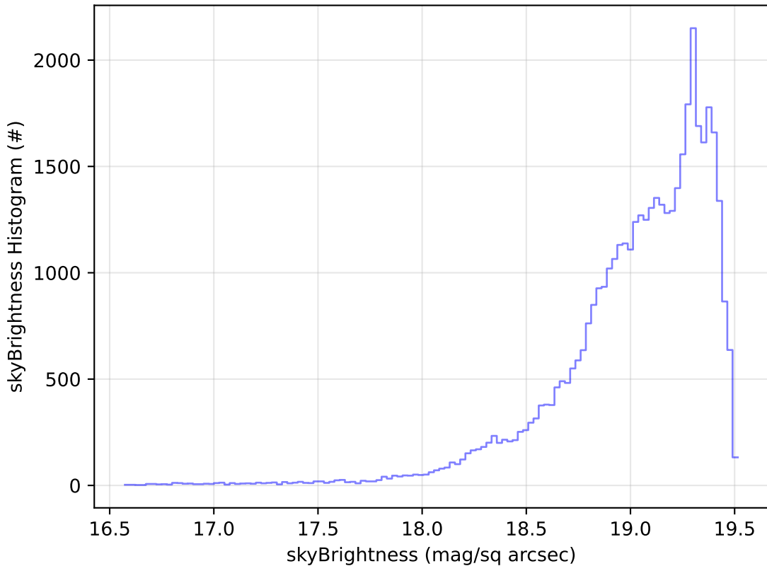
too_elab_r128_d2_gz_v3.4_10yrs Yr 1 z band: skyBrightness Histogram
