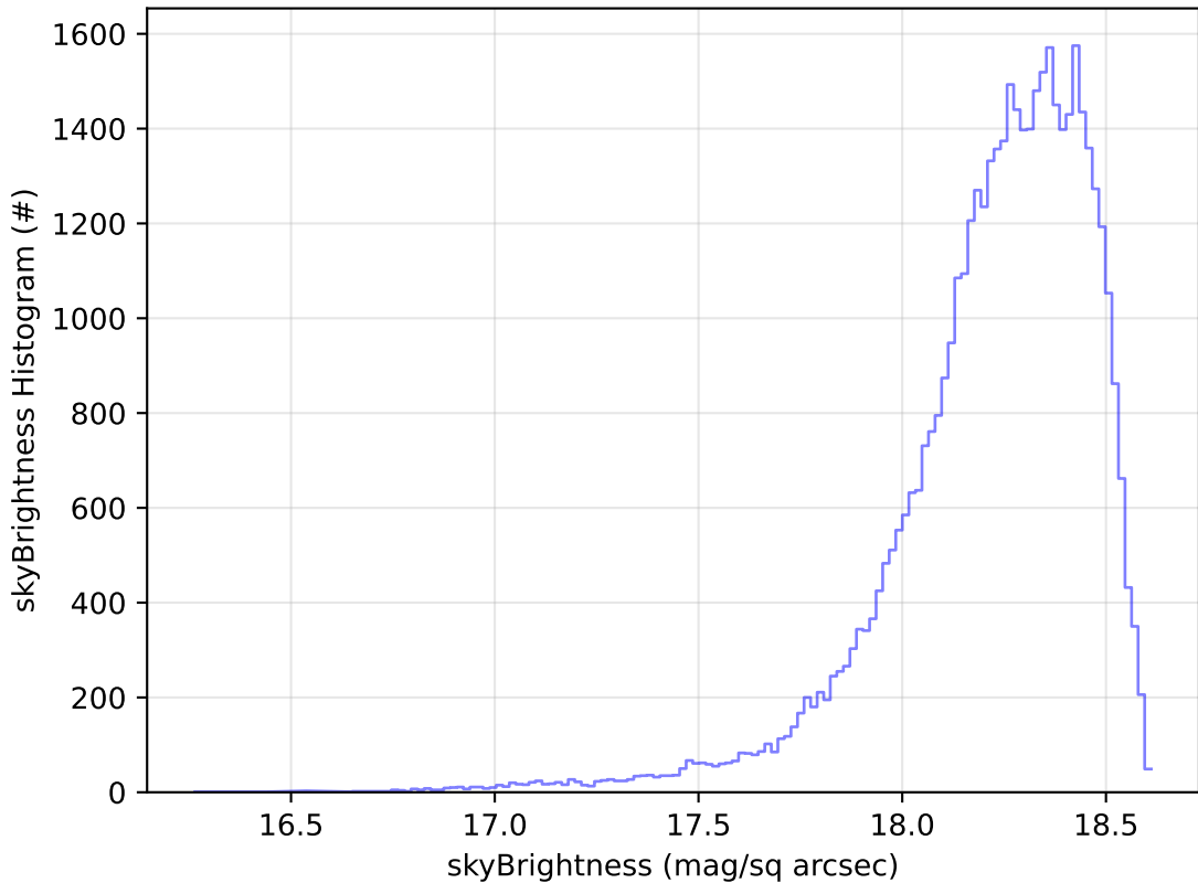
too_elab_r128_d2_gz_v3.4_10yrs Yr 1 y band: skyBrightness Histogram
