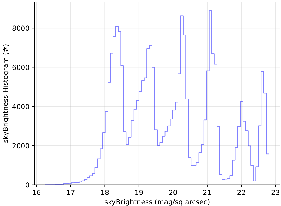
too_elab_r128_d2_gz_v3.4_10yrs Yr 1 all bands: skyBrightness Histogram
