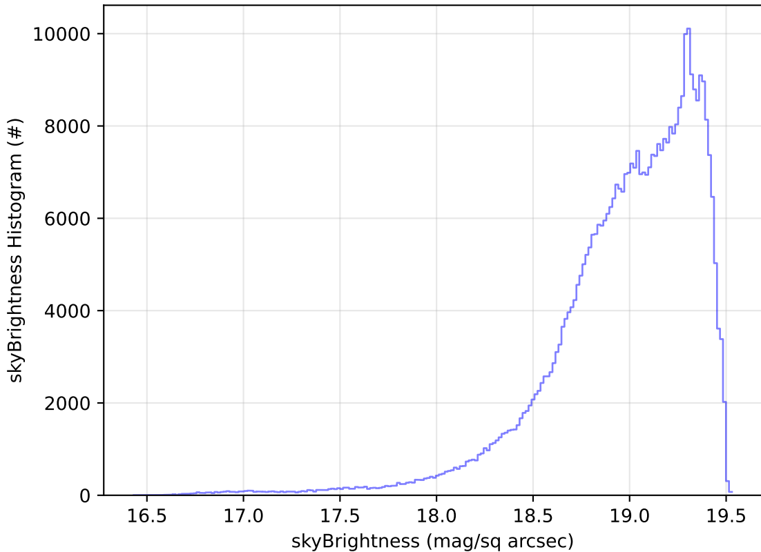
too_elab_r128_d2_gz_v3.4_10yrs WFD z band: skyBrightness Histogram
