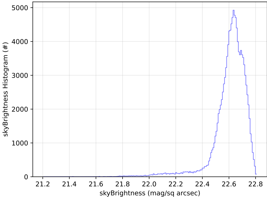
too_elab_r128_d2_gz_v3.4_10yrs WFD u band: skyBrightness Histogram
