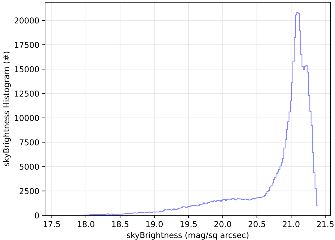
too_elab_r128_d2_gz_v3.4_10yrs WFD r band: skyBrightness Histogram
