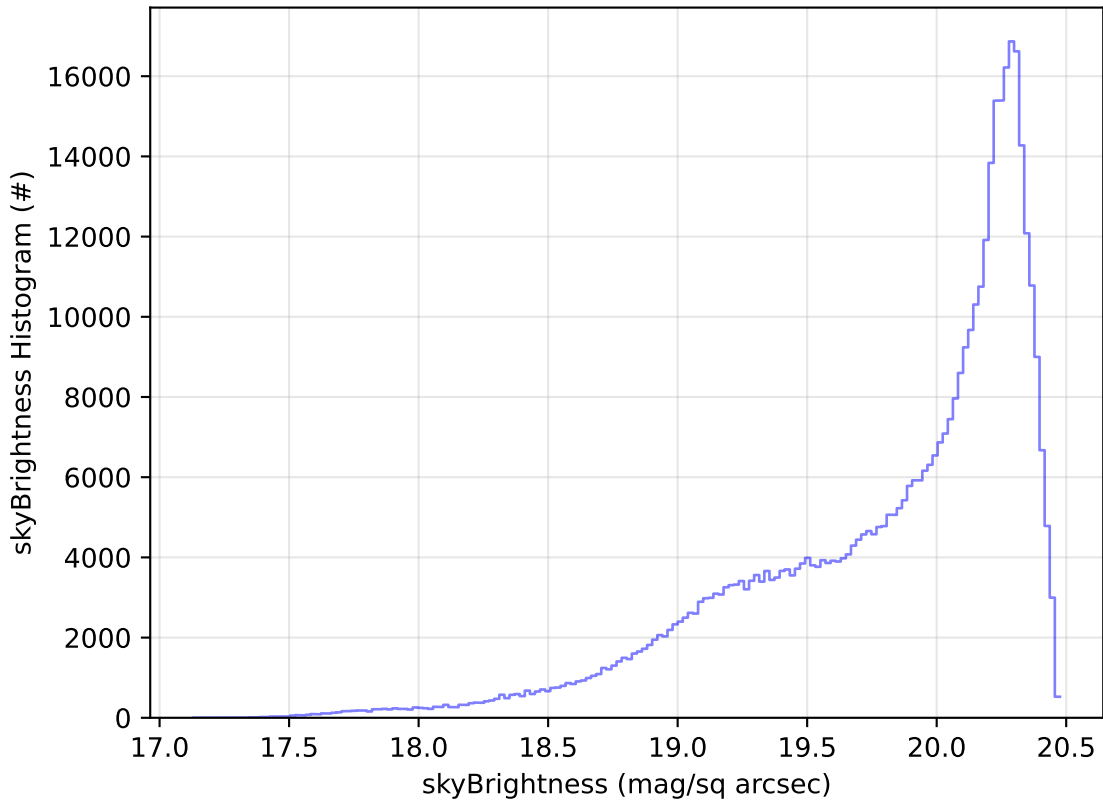
too_elab_r128_d2_gz_v3.4_10yrs WFD i band: skyBrightness Histogram
