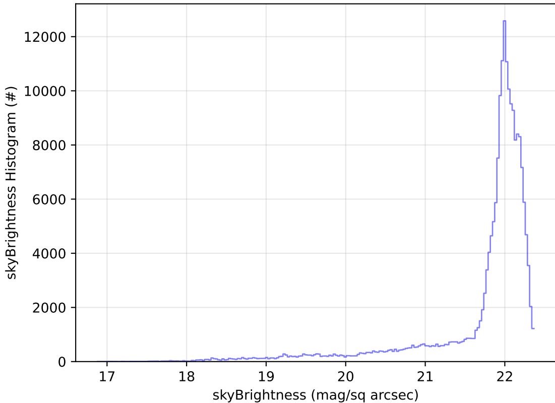
too_elab_r128_d2_gz_v3.4_10yrs WFD g band: skyBrightness Histogram
