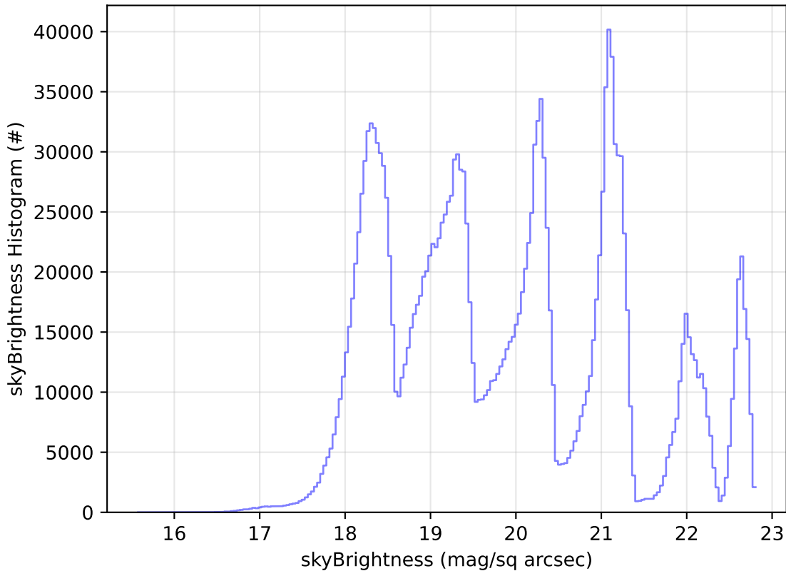
too_elab_r128_d2_gz_v3.4_10yrs WFD all bands: skyBrightness Histogram
