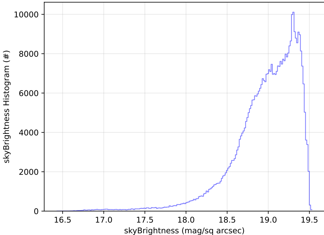
too_elab_r128_d2_gz_v3.4_10yrs All sky z band: skyBrightness Histogram
