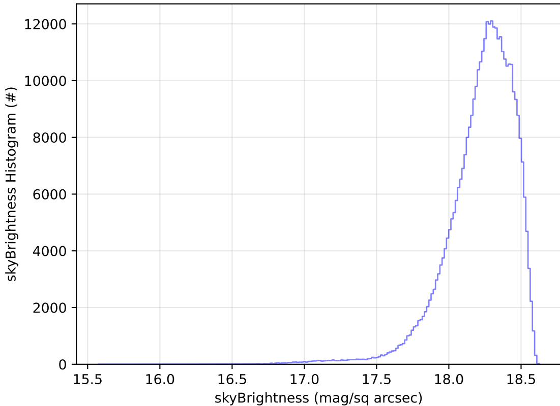
too_elab_r128_d2_gz_v3.4_10yrs All sky y band: skyBrightness Histogram
