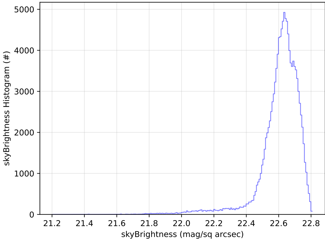
too_elab_r128_d2_gz_v3.4_10yrs All sky u band: skyBrightness Histogram
