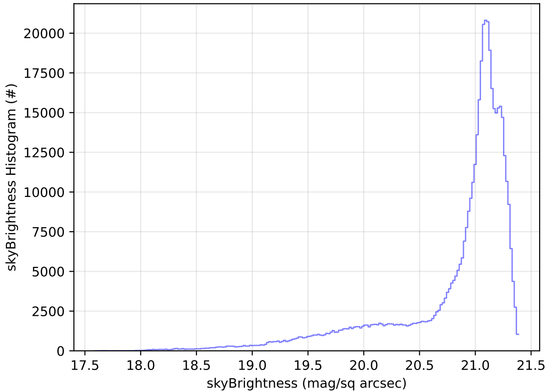
too_elab_r128_d2_gz_v3.4_10yrs All sky r band: skyBrightness Histogram
