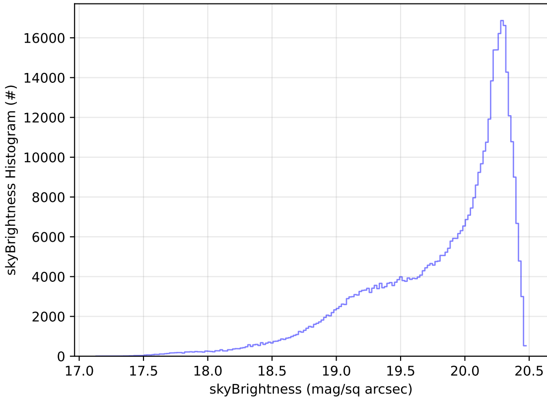
too_elab_r128_d2_gz_v3.4_10yrs All sky i band: skyBrightness Histogram
