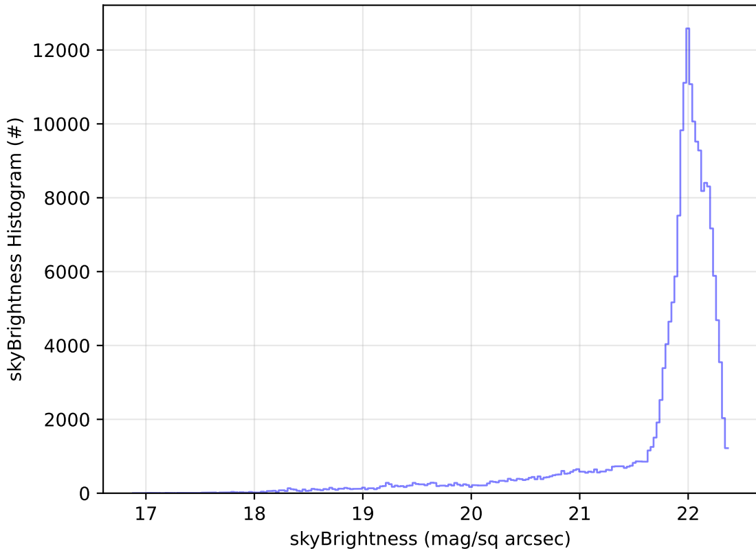
too_elab_r128_d2_gz_v3.4_10yrs All sky g band: skyBrightness Histogram
