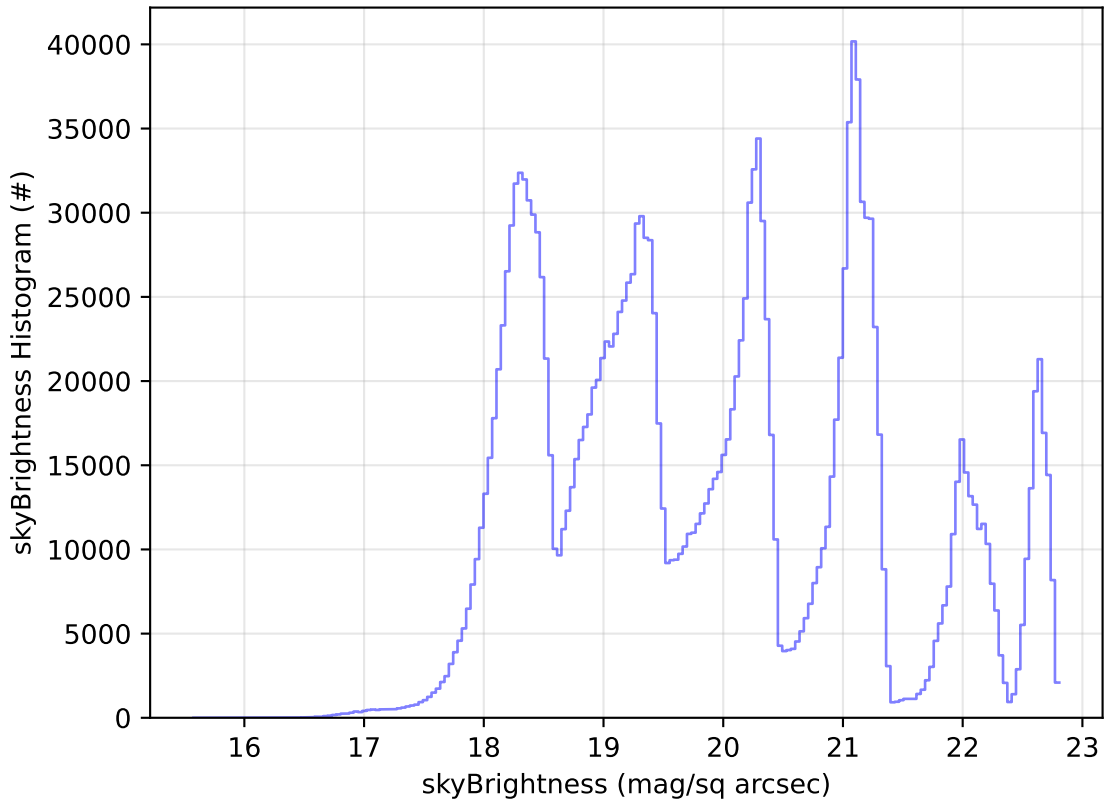
too_elab_r128_d2_gz_v3.4_10yrs All sky all bands: skyBrightness Histogram
