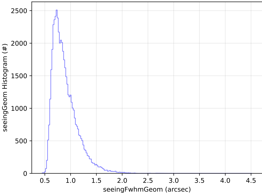
too_elab_r128_d2_gz_v3.4_10yrs Yr 1 r band: seeingGeom Histogram
