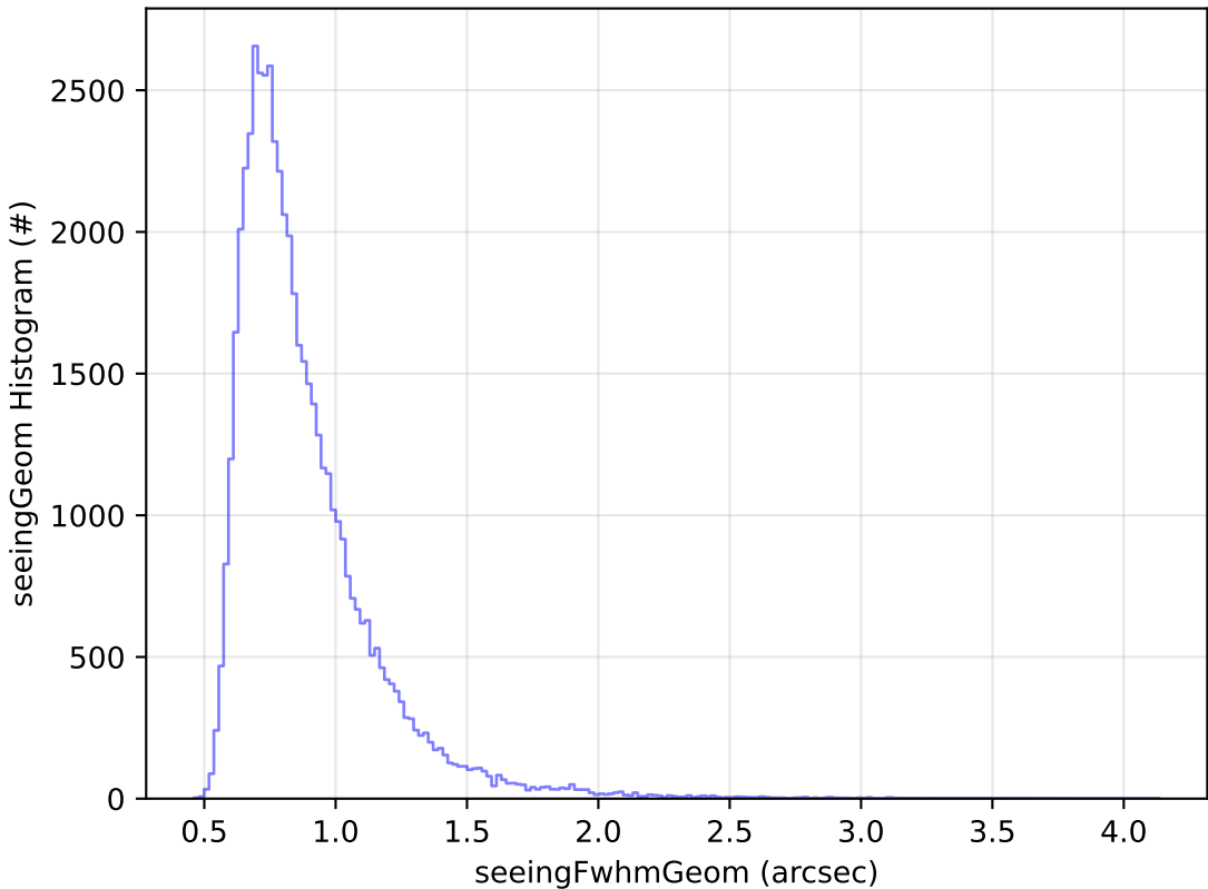
too_elab_r128_d2_gz_v3.4_10yrs Yr 1 i band: seeingGeom Histogram
