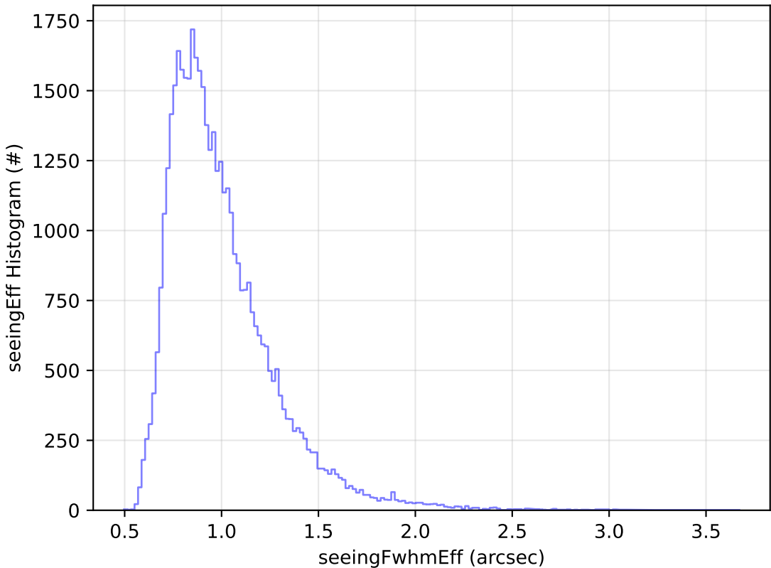
too_elab_r128_d2_gz_v3.4_10yrs Yr 1 z band: seeingEff Histogram
