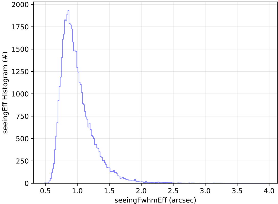
too_elab_r128_d2_gz_v3.4_10yrs Yr 1 y band: seeingEff Histogram
