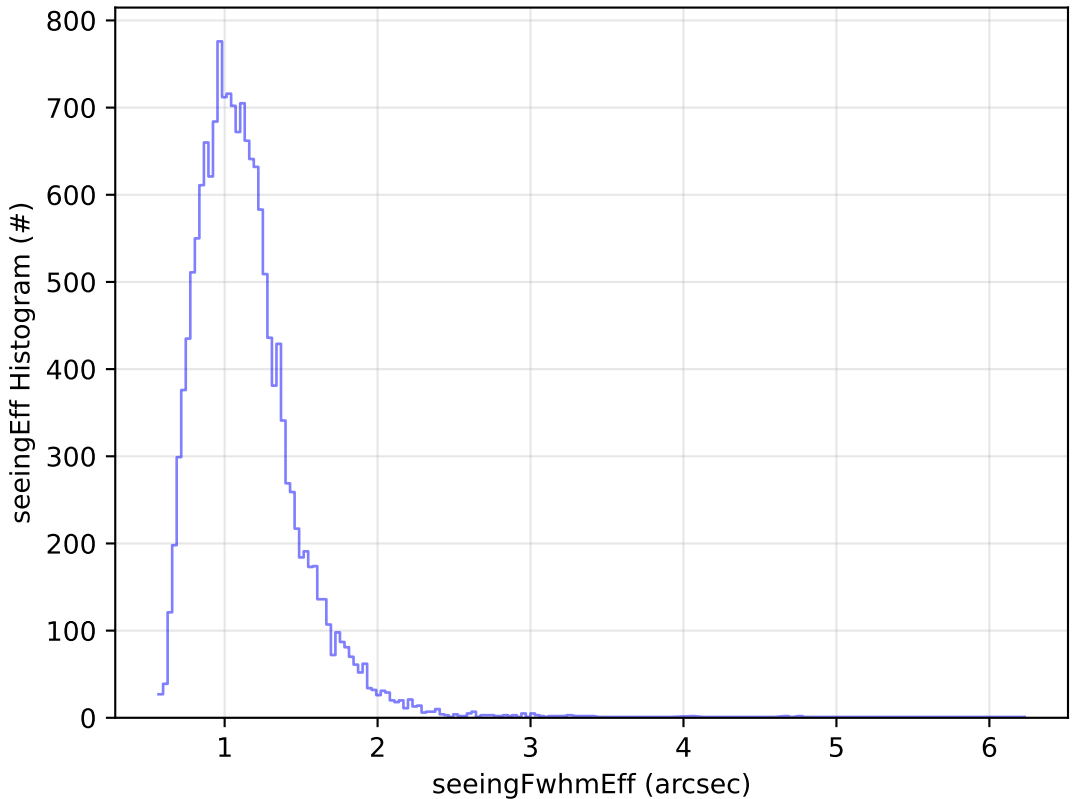
too_elab_r128_d2_gz_v3.4_10yrs Yr 1 u band: seeingEff Histogram
