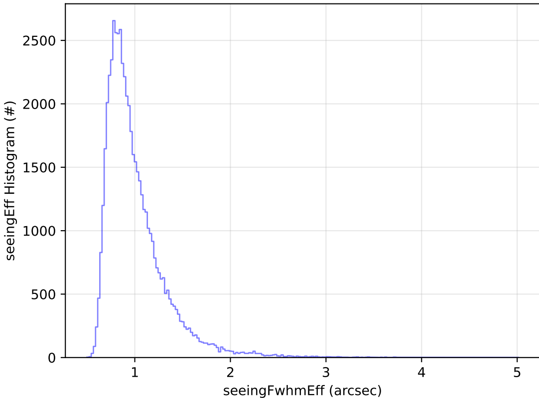
too_elab_r128_d2_gz_v3.4_10yrs Yr 1 i band: seeingEff Histogram
