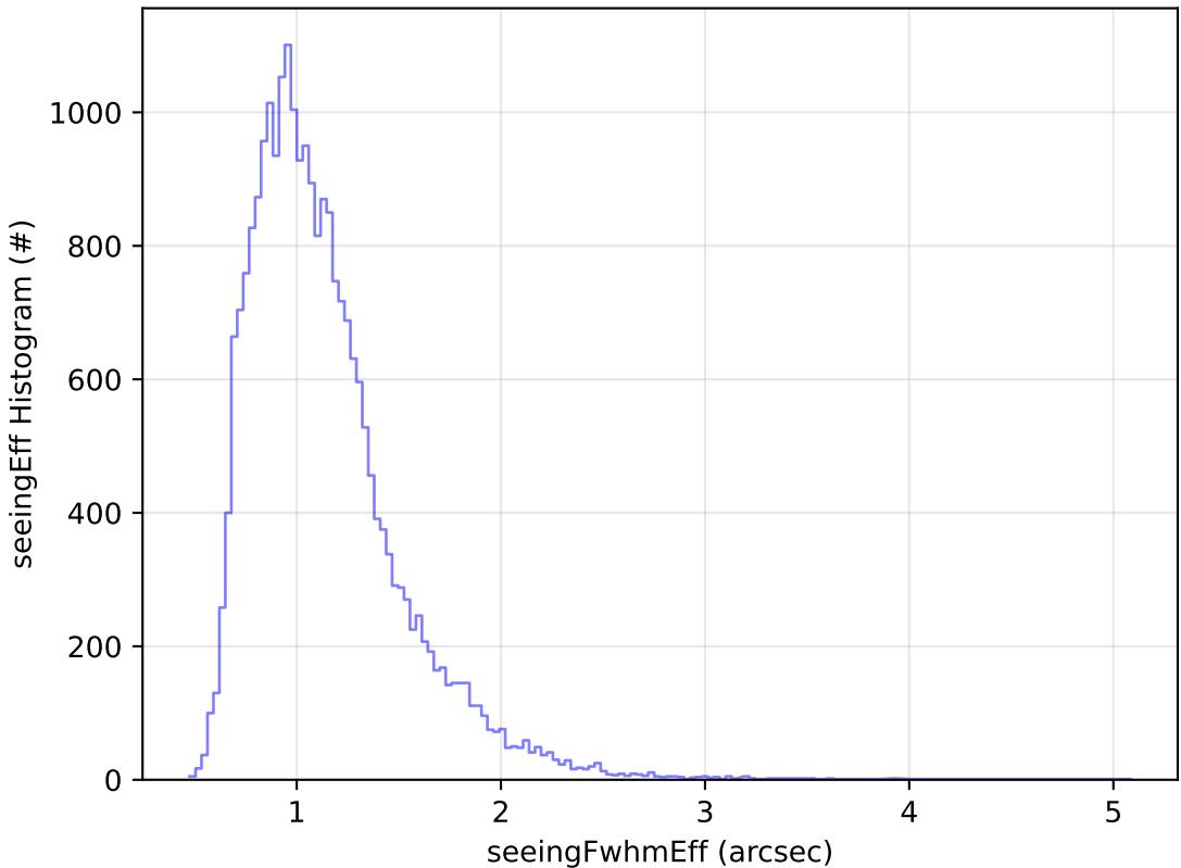
too_elab_r128_d2_gz_v3.4_10yrs Yr 1 g band: seeingEff Histogram
