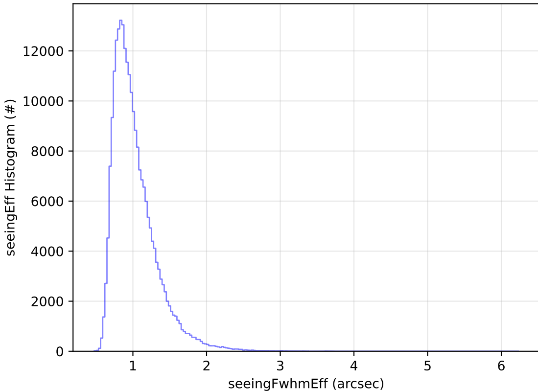
too_elab_r128_d2_gz_v3.4_10yrs Yr 1 all bands: seeingEff Histogram
