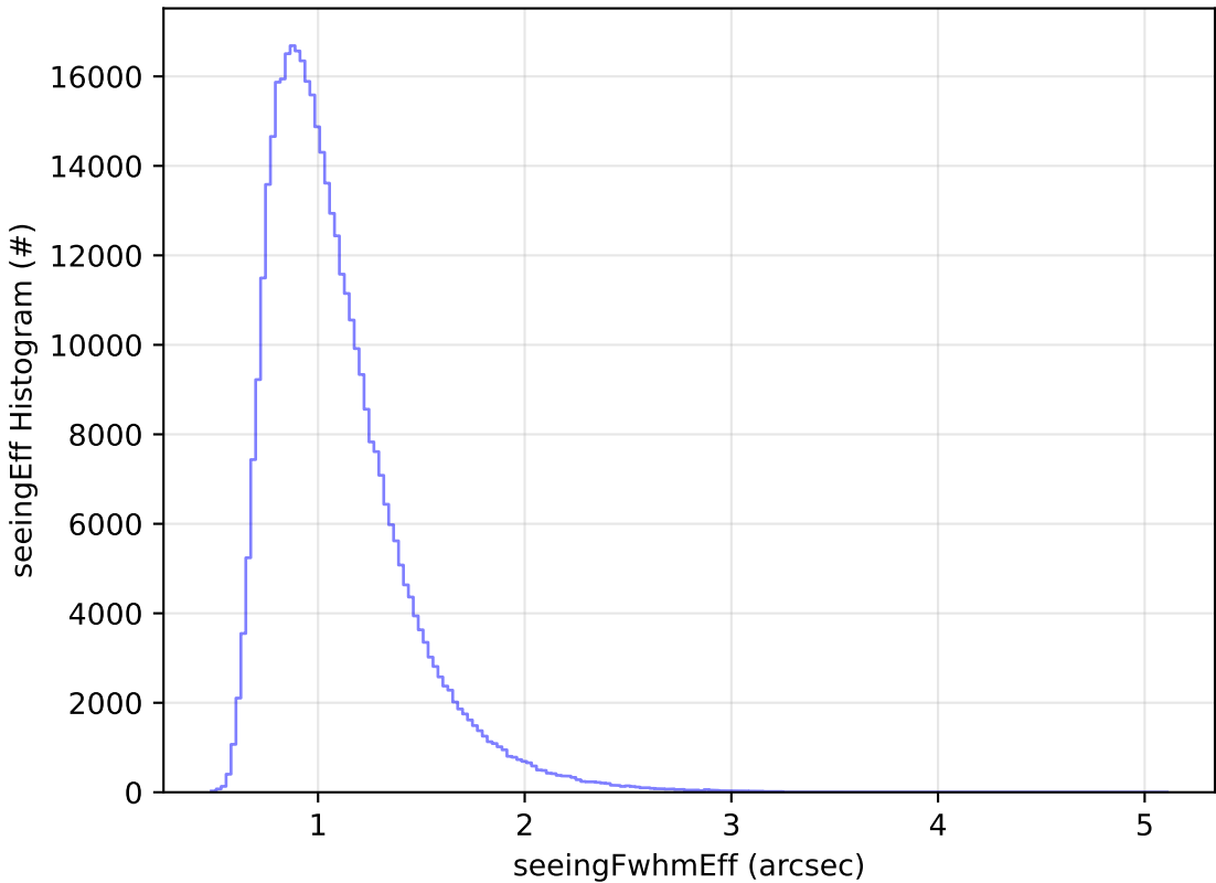
too_elab_r128_d2_gz_v3.4_10yrs WFD z band: seeingEff Histogram
