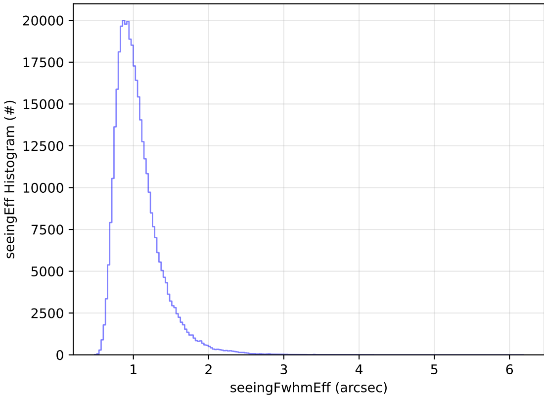
too_elab_r128_d2_gz_v3.4_10yrs WFD y band: seeingEff Histogram
