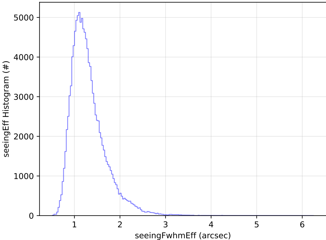
too_elab_r128_d2_gz_v3.4_10yrs WFD u band: seeingEff Histogram
