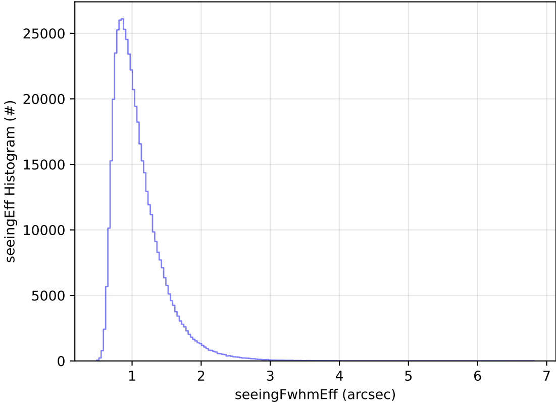
too_elab_r128_d2_gz_v3.4_10yrs WFD i band: seeingEff Histogram
