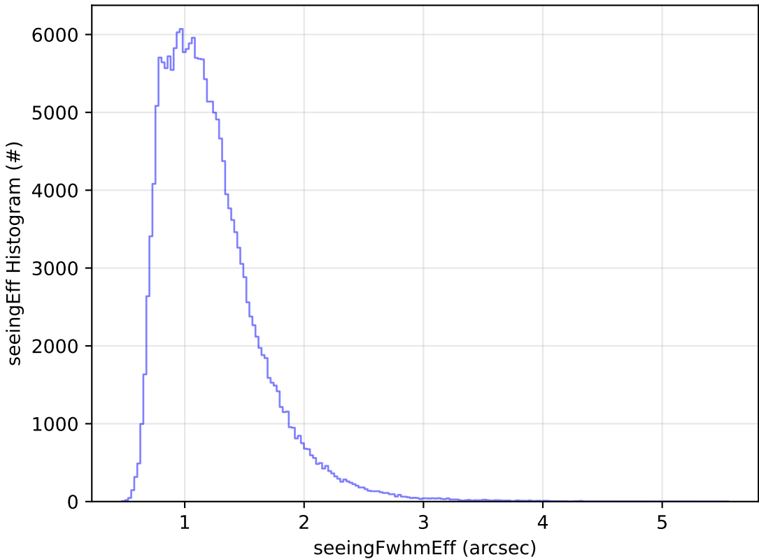
too_elab_r128_d2_gz_v3.4_10yrs WFD g band: seeingEff Histogram
