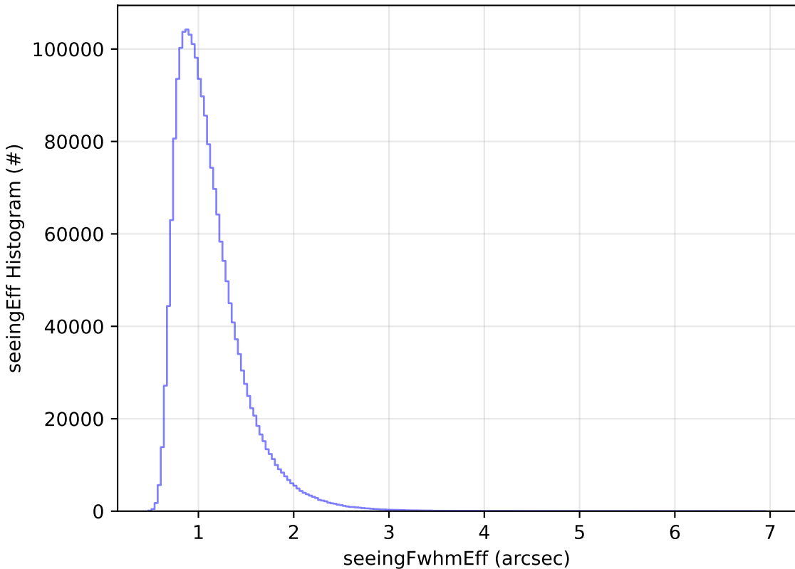
too_elab_r128_d2_gz_v3.4_10yrs WFD all bands: seeingEff Histogram
