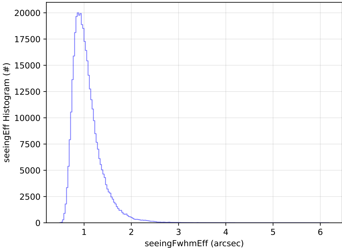
too_elab_r128_d2_gz_v3.4_10yrs All sky y band: seeingEff Histogram
