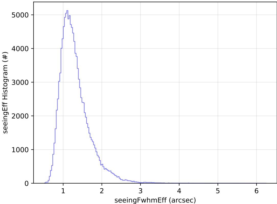
too_elab_r128_d2_gz_v3.4_10yrs All sky u band: seeingEff Histogram
