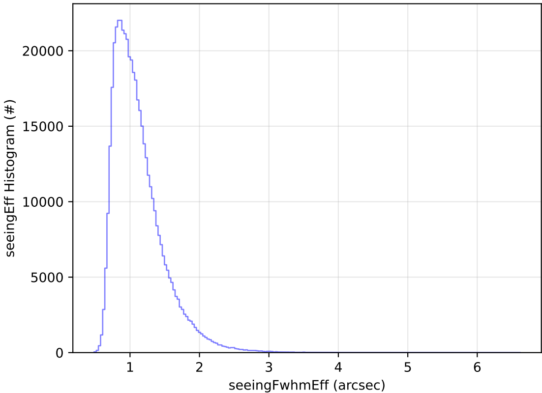
too_elab_r128_d2_gz_v3.4_10yrs All sky r band: seeingEff Histogram
