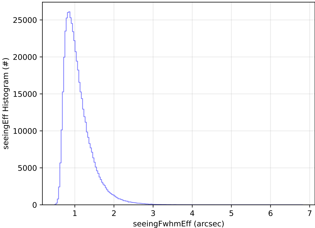
too_elab_r128_d2_gz_v3.4_10yrs All sky i band: seeingEff Histogram
