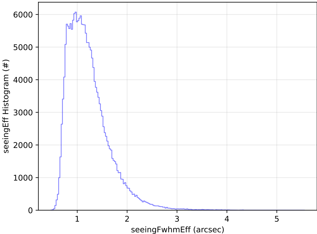
too_elab_r128_d2_gz_v3.4_10yrs All sky g band: seeingEff Histogram
