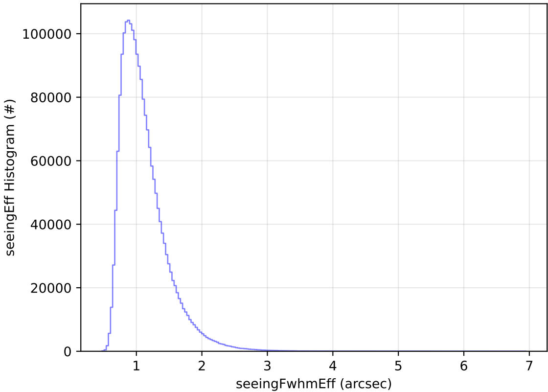
too_elab_r128_d2_gz_v3.4_10yrs All sky all bands: seeingEff Histogram
