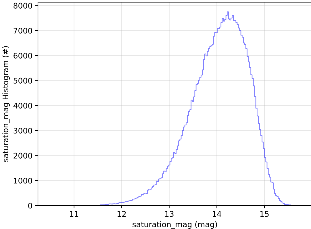
too_elab_r128_d2_gz_v3.4_10yrs WFD z band: saturation_mag Histogram
