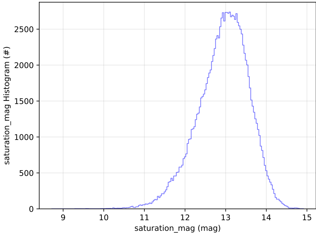
too_elab_r128_d2_gz_v3.4_10yrs WFD u band: saturation_mag Histogram
