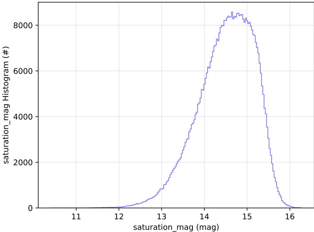
too_elab_r128_d2_gz_v3.4_10yrs WFD r band: saturation_mag Histogram
