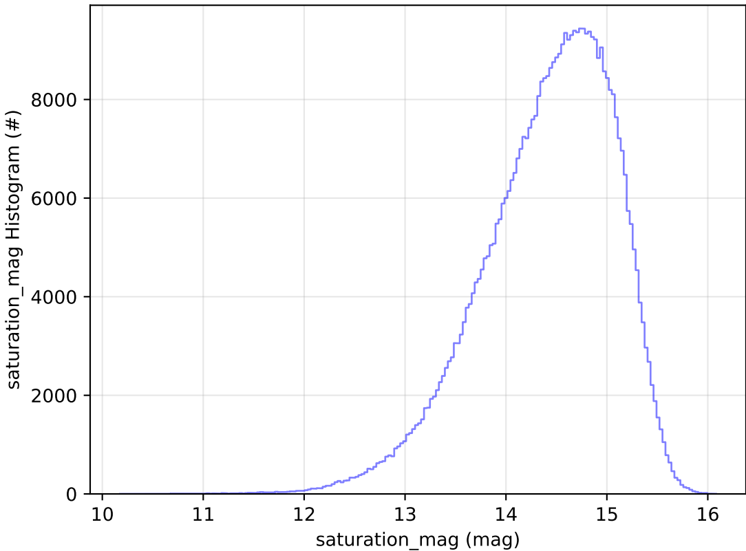
too_elab_r128_d2_gz_v3.4_10yrs WFD i band: saturation_mag Histogram
