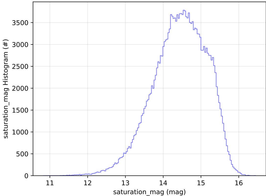
too_elab_r128_d2_gz_v3.4_10yrs WFD g band: saturation_mag Histogram
