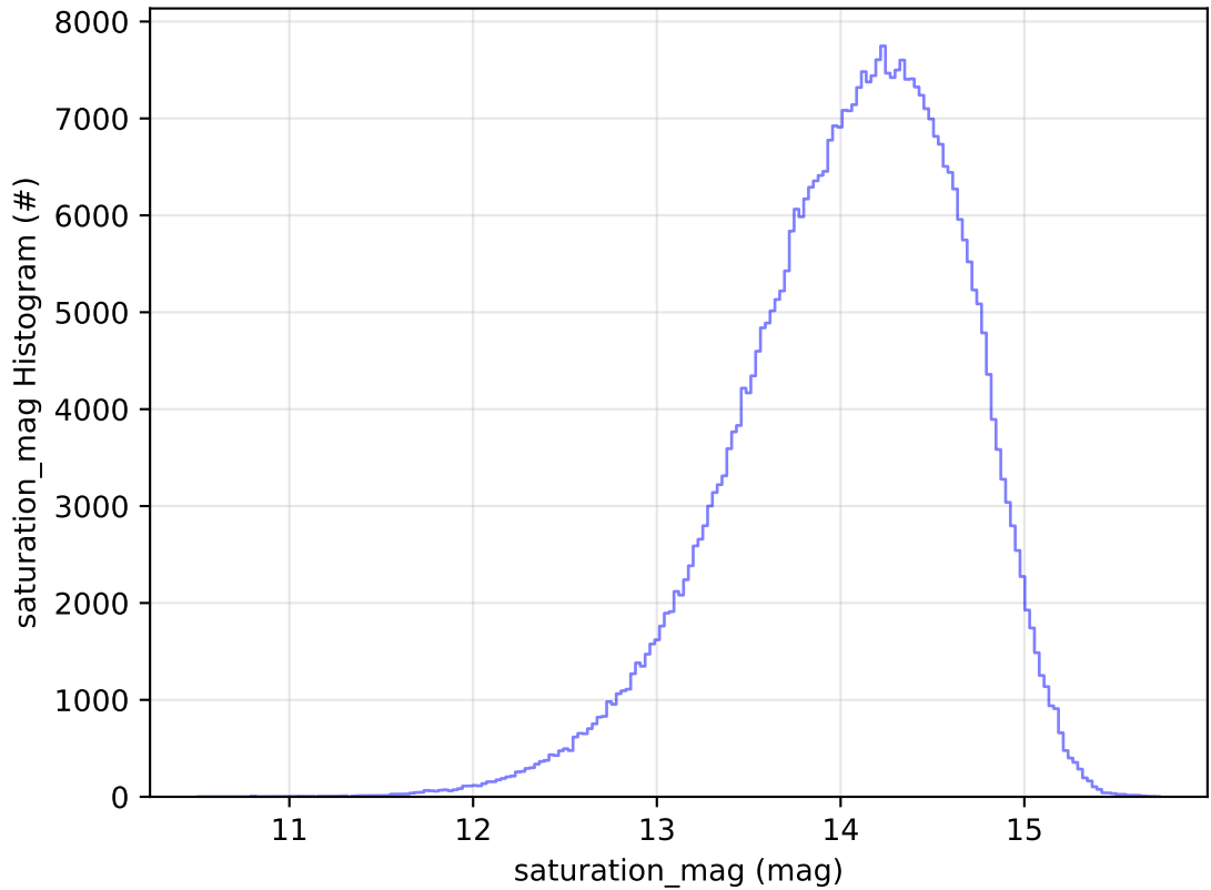
too_elab_r128_d2_gz_v3.4_10yrs All sky z band: saturation_mag Histogram
