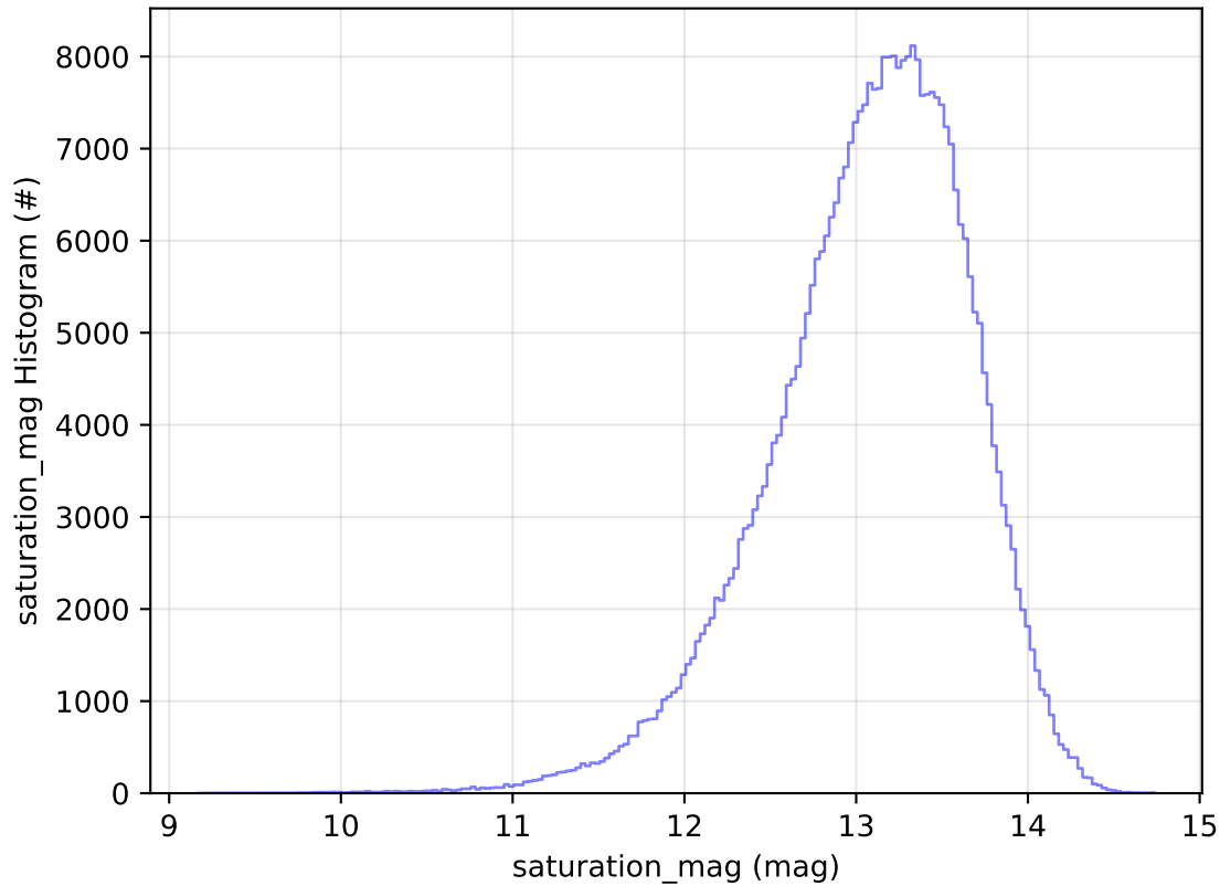
too_elab_r128_d2_gz_v3.4_10yrs All sky y band: saturation_mag Histogram
