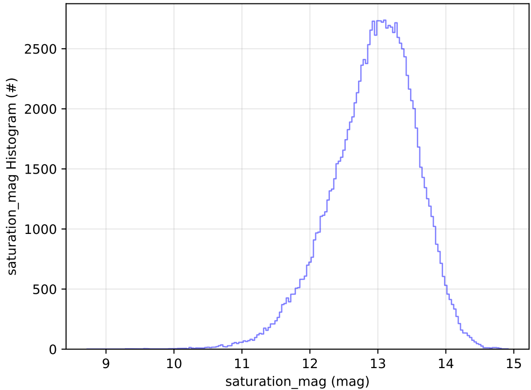
too_elab_r128_d2_gz_v3.4_10yrs All sky u band: saturation_mag Histogram
