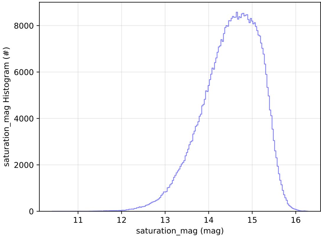
too_elab_r128_d2_gz_v3.4_10yrs All sky r band: saturation_mag Histogram
